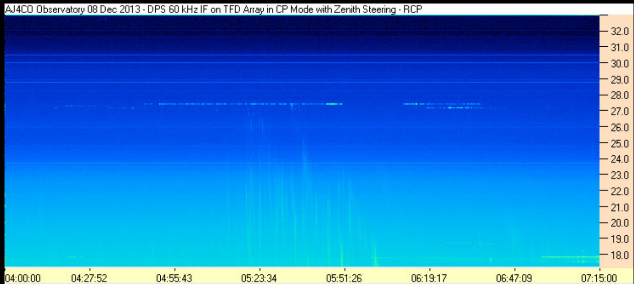
Io-A 131208040000AJ4CO DPS.PNG
