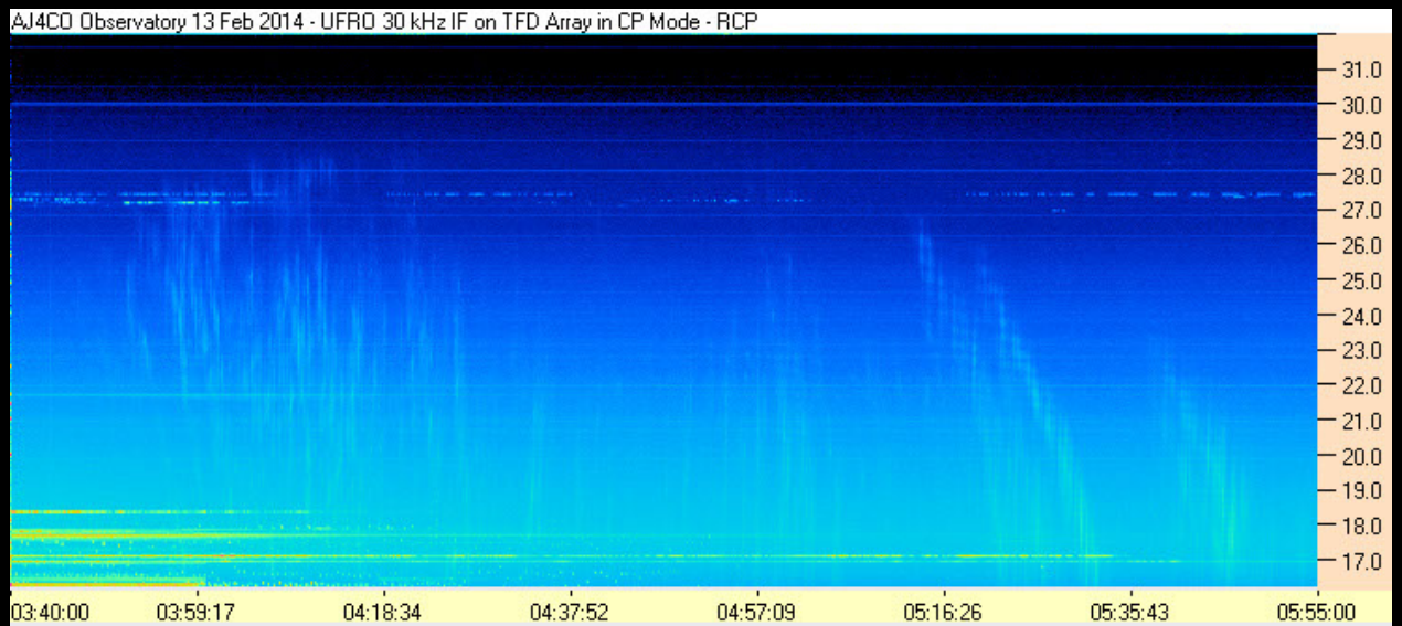
Io-A 140213034000AJ4CO DPS.PNG
