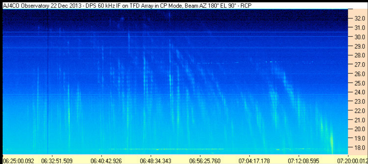
Io-A 131222062500AJ4CO DPS.PNG
