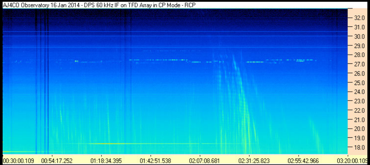
Io-A 140116003000AJ4CO DPS.PNG
