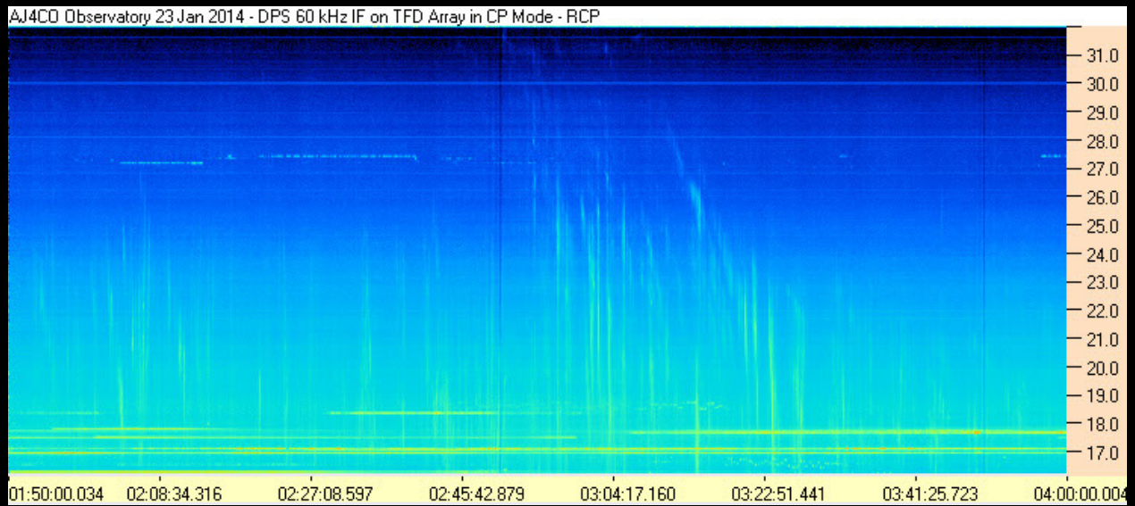
Io-A 140123015000AJ4CO DPS.PNG
