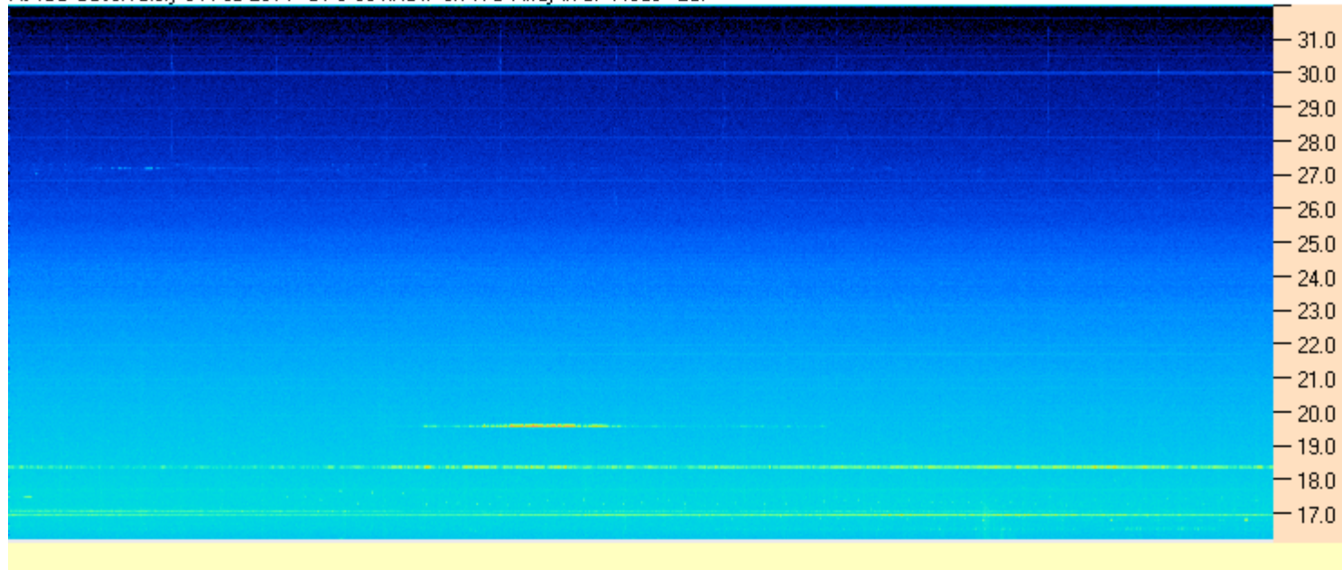
AJ4CO Observatory 04 Feb 2014 - DPS 60 kHz IF on TFD Array in CP Mode - LCP
