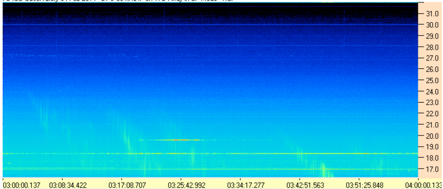
AJ4CO Observatory 04 Feb 2014 - DPS 60 kHz IF on TFD Array in CP Mode - RCP
