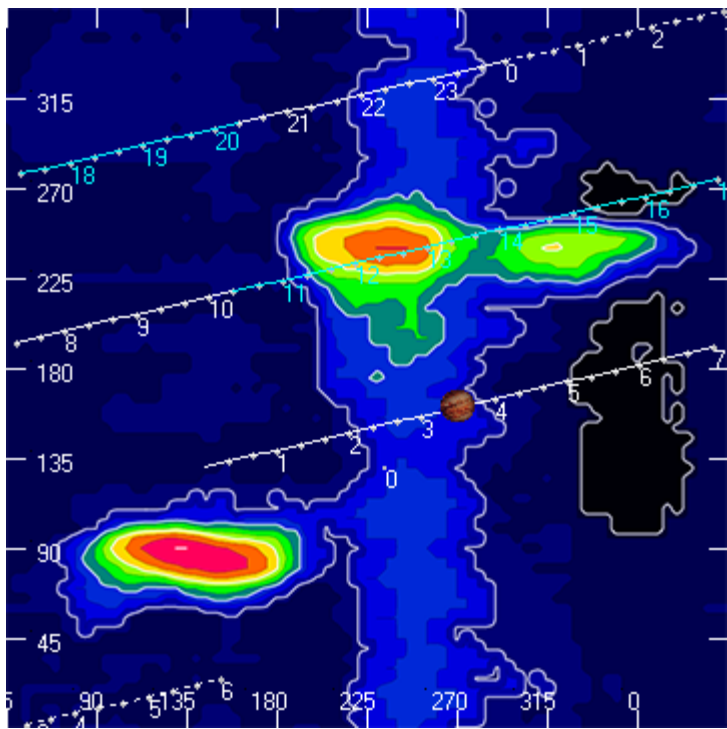
AJ4CO Observatory 04 Feb 2014 - DPS 60 kHz IF on TFD Array in CP Mode - RCP
