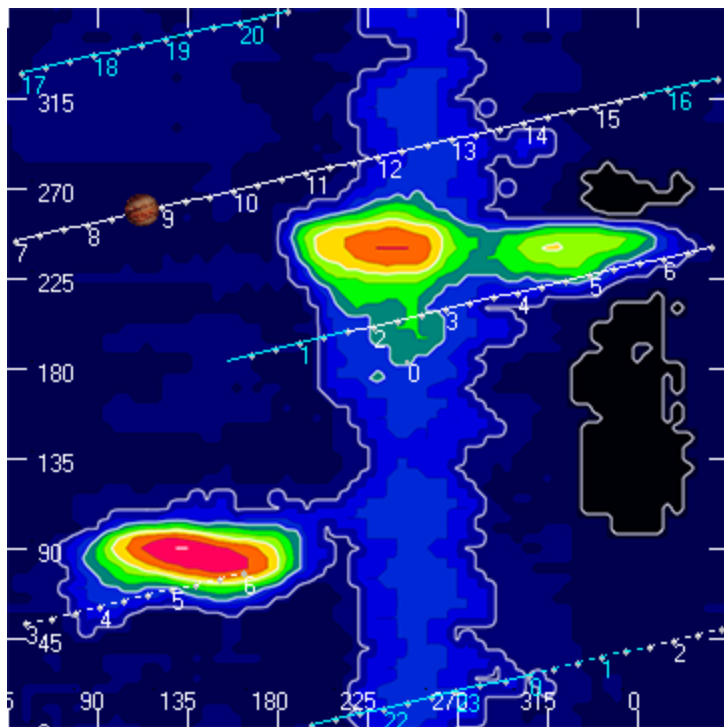
AJ4CD Observatory 22 Nov 2013 - DPS 60 kHz IF on TFD Array
