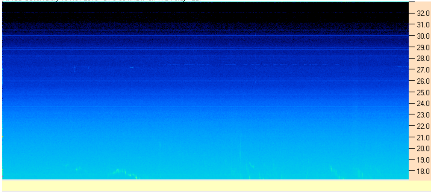
AJ4CO Observatory 15 Nov 2013 - DPS 60 kHz IF on TFD Array - LCP
