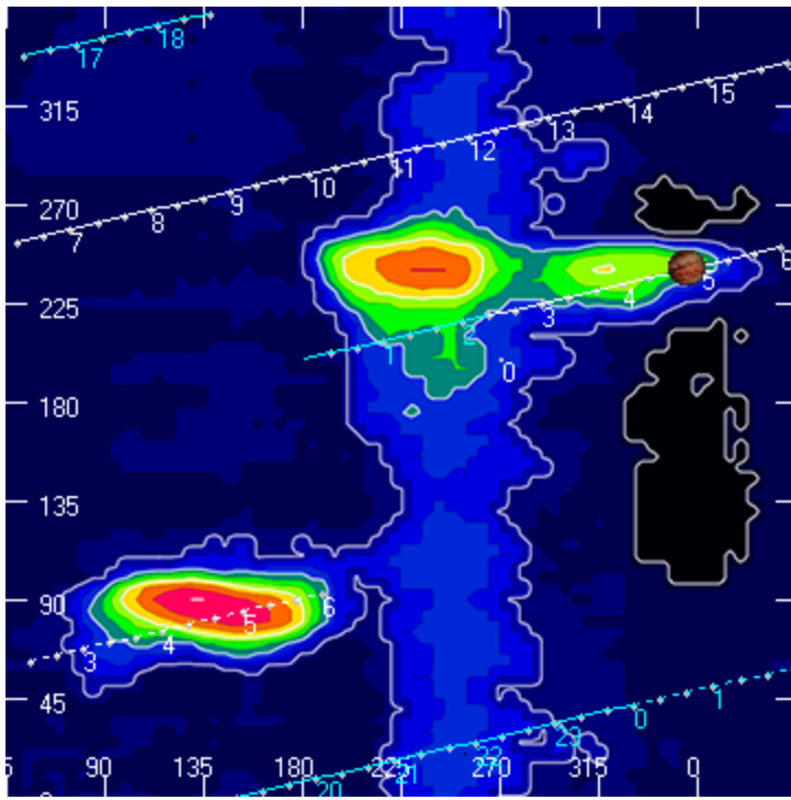
AJ4CD Observatory 15 Nov 2013 - DPS 60 kHz IF on TFD Array - RCP
